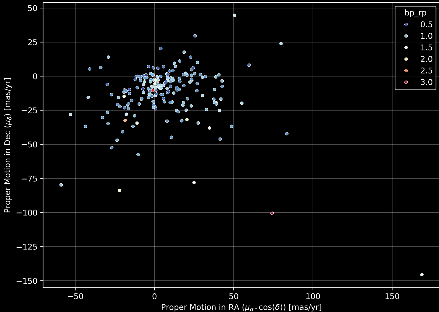
APOGEE DR17 Field: [K2_C3_051-52] Proper Motion Diagram (n= 195)
