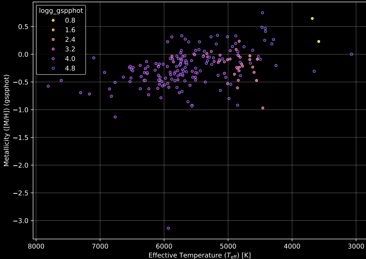
APOGEE DR17 Field: [K2_C3_051-52] Stellar Population Parameters (n= 195)
