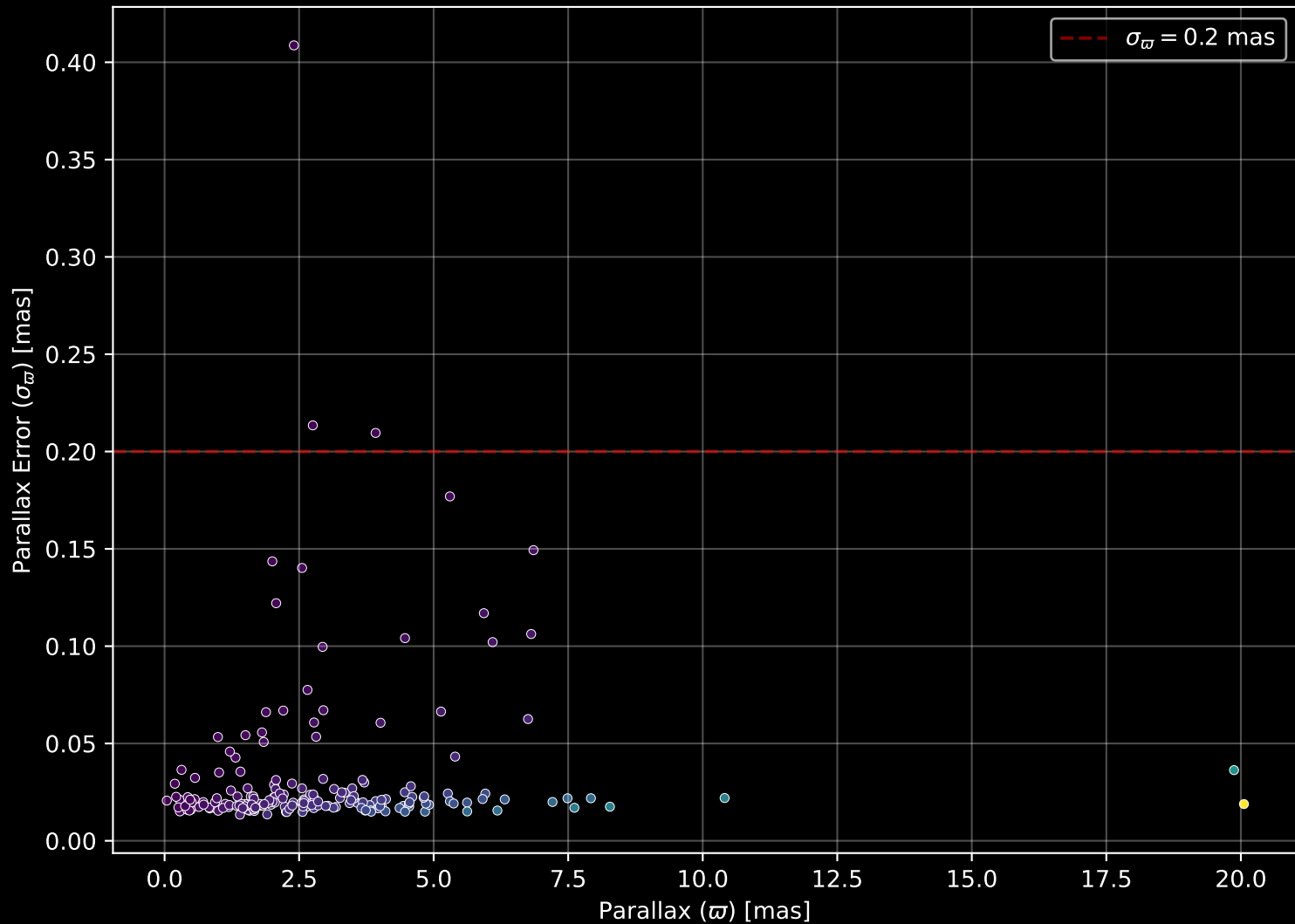
APOGEE DR17 Field: [K2 C3 051-52] Parallax Quality (n= 195)
