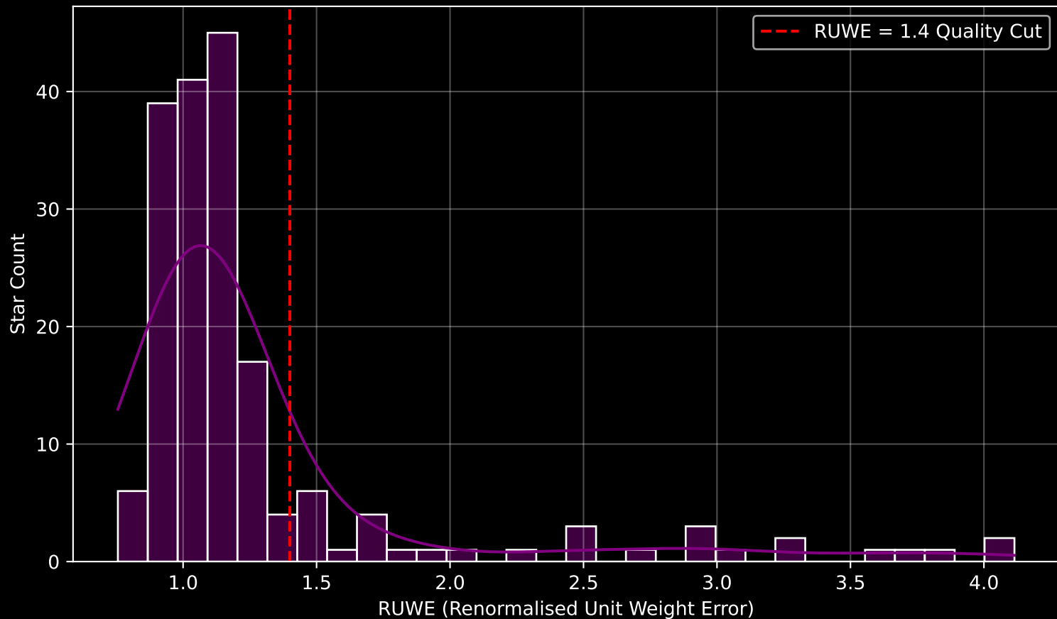
GAPOGEE DR17 Field [K2_C3_051-52] RUWE Distribution (n= 182)
