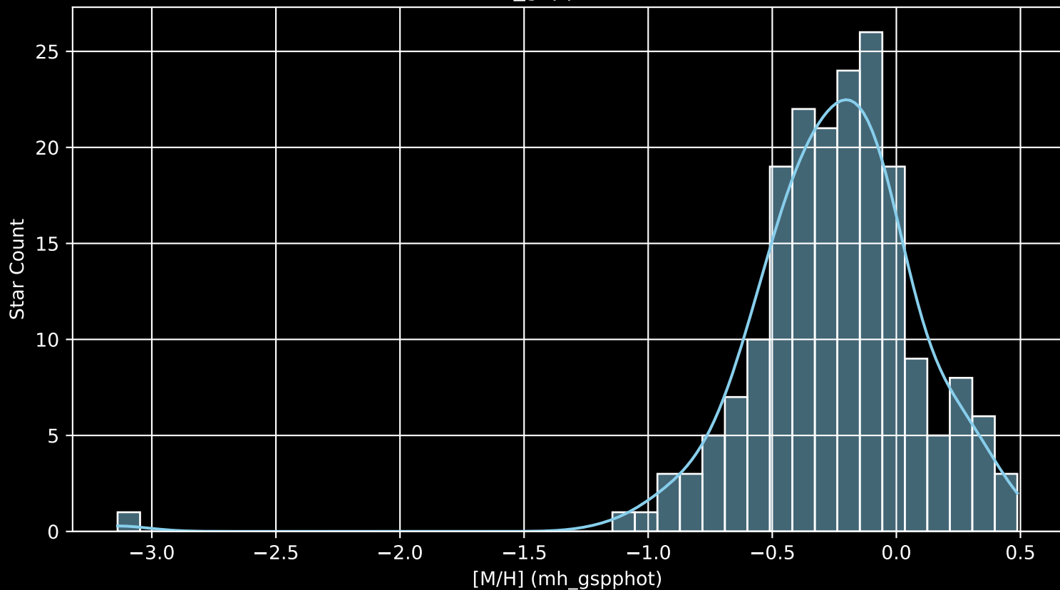
APOGEE DR17 Field: [K2_C3_051-52 [M/H] (mh_gspphot) (n= 193)
