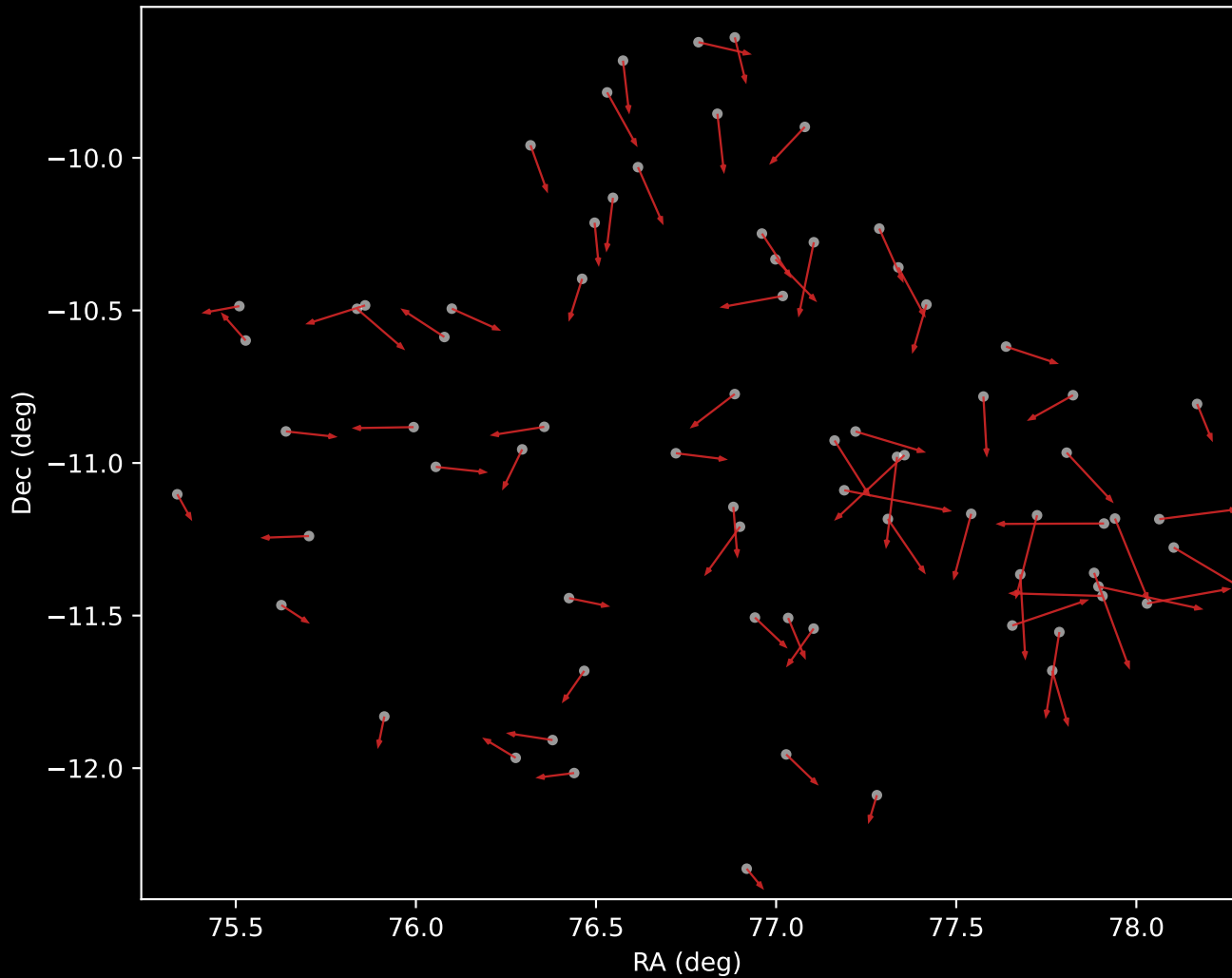
APOGEE DR17 Cluster 6 Proper Motion Vectors (n=73)
