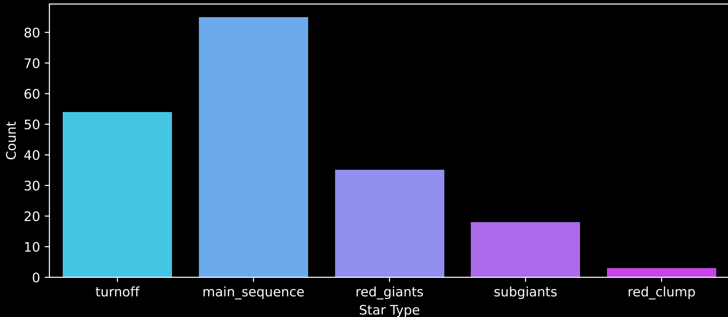
APOGEE DR17 Field: [K2_C3_051-52] Count plot of Star Type
